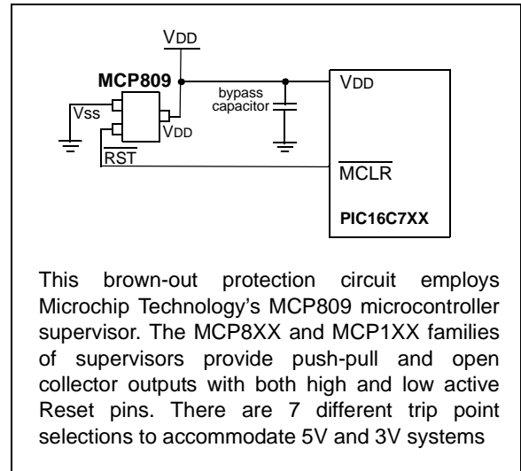
FIGURE 9-10: EXTERNAL BROWN-OUT PROTECTION CIRCUIT 3
